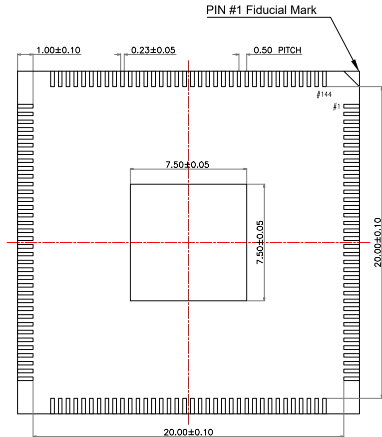
BOTTOM VIEW
